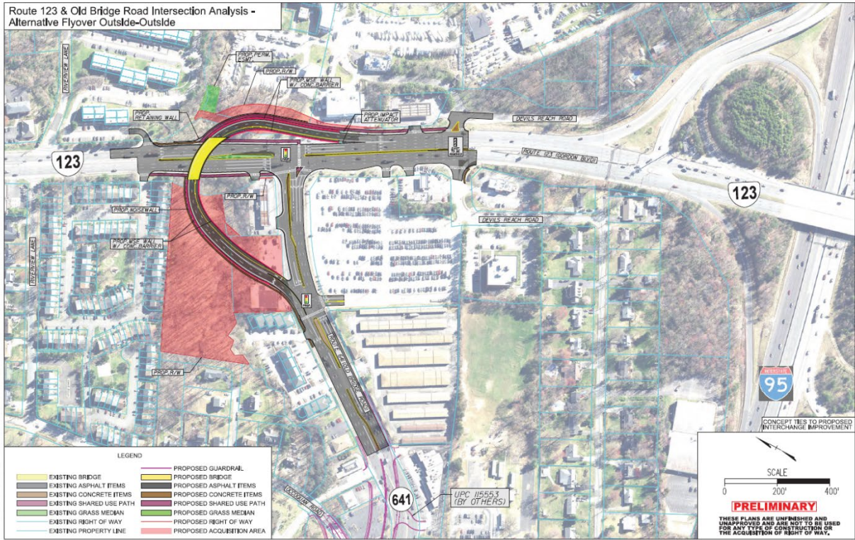
Figure 4: Route 123 at Old Bridge Flyover Concept
