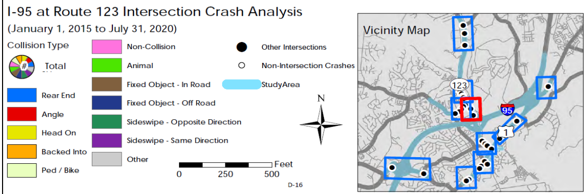
Figure 10. Project Area Crash Analysis
