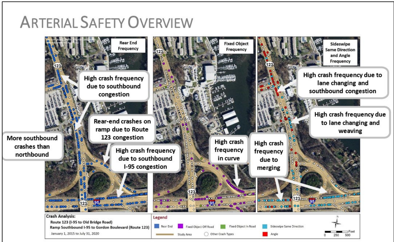
Figure 9. Project Area Safety Overview
